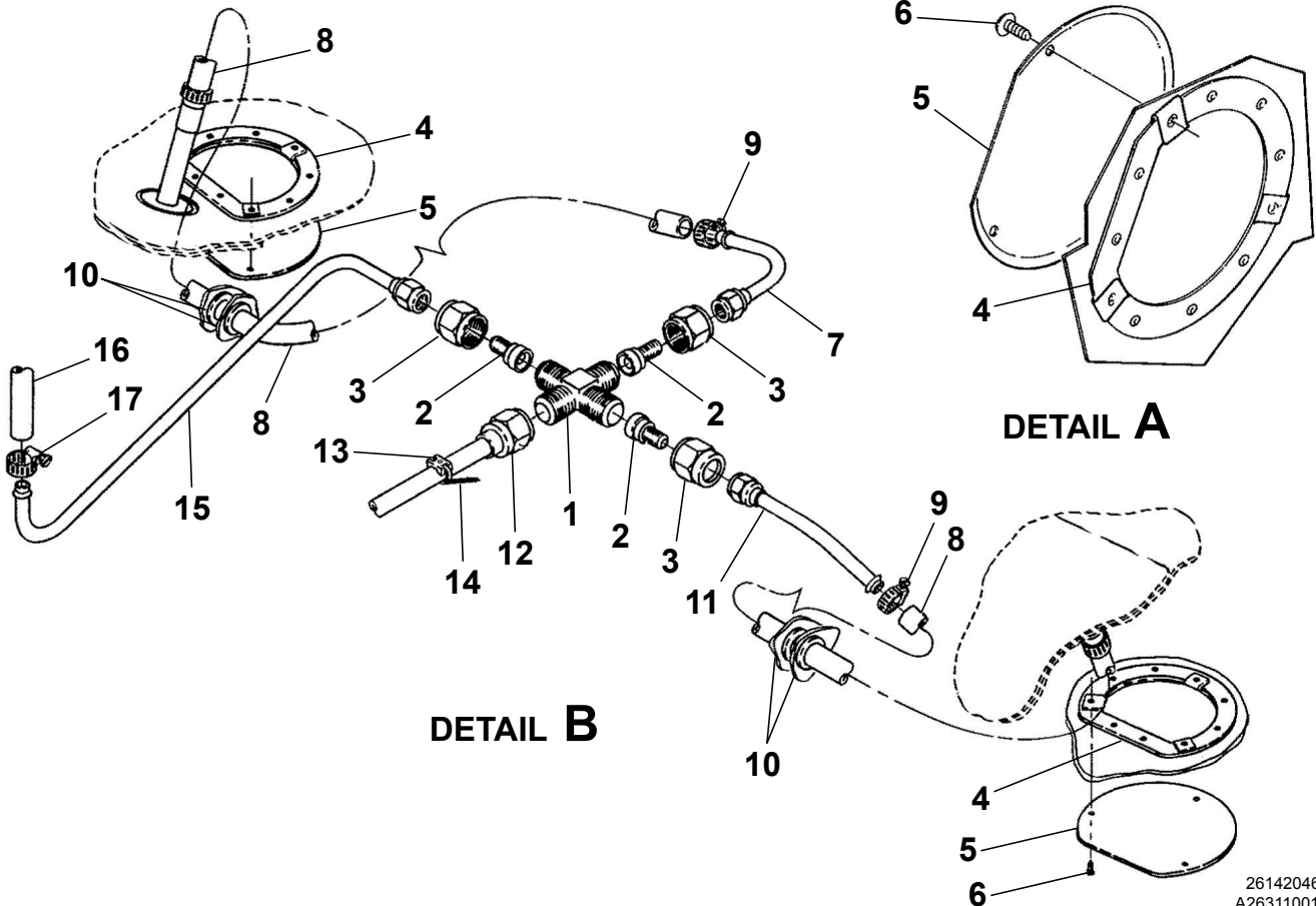
DEICE COMPONENTS - STABILIZER Figure 01. (Sheet 1)
