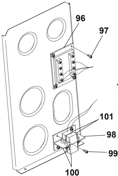
DETAIL C
