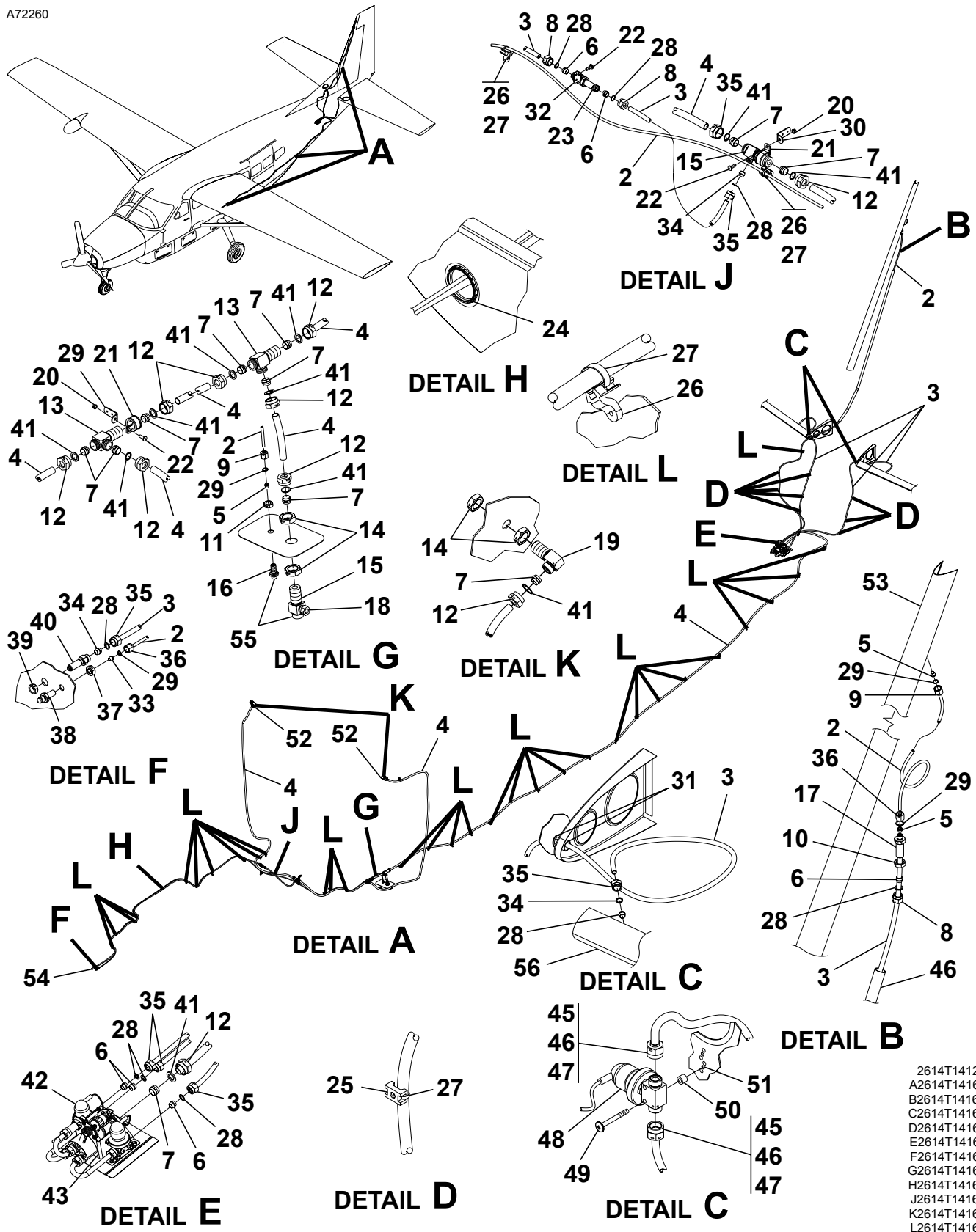
TKS TUBE ROUTING - FUSELAGE Figure 04. (Sheet 1)
