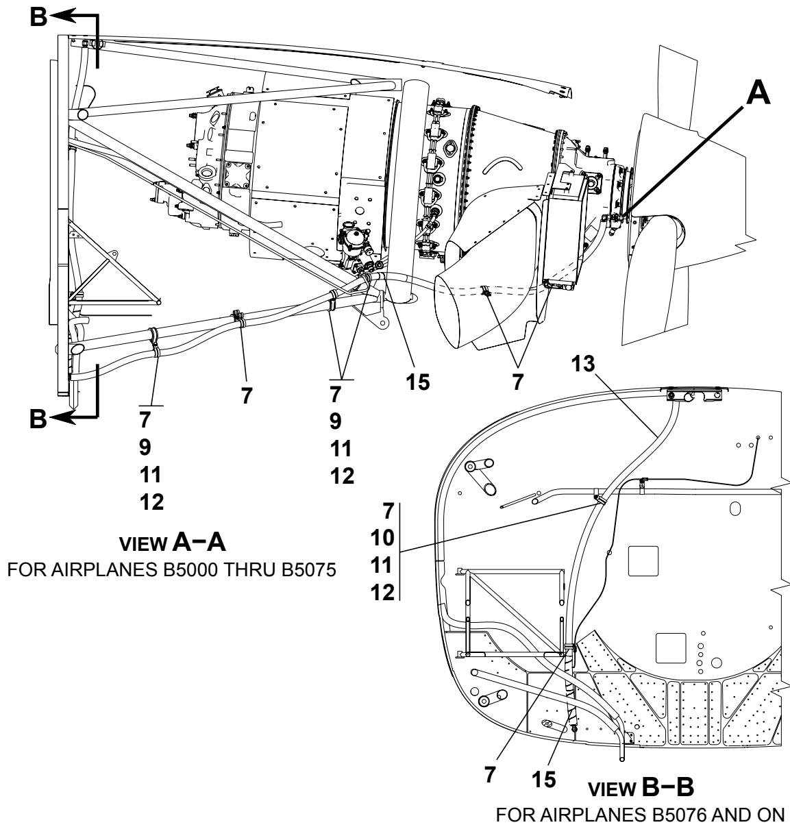
TKS FIREWALL FORWARD INSTALLATION Figure 05A. (Sheet 1)
