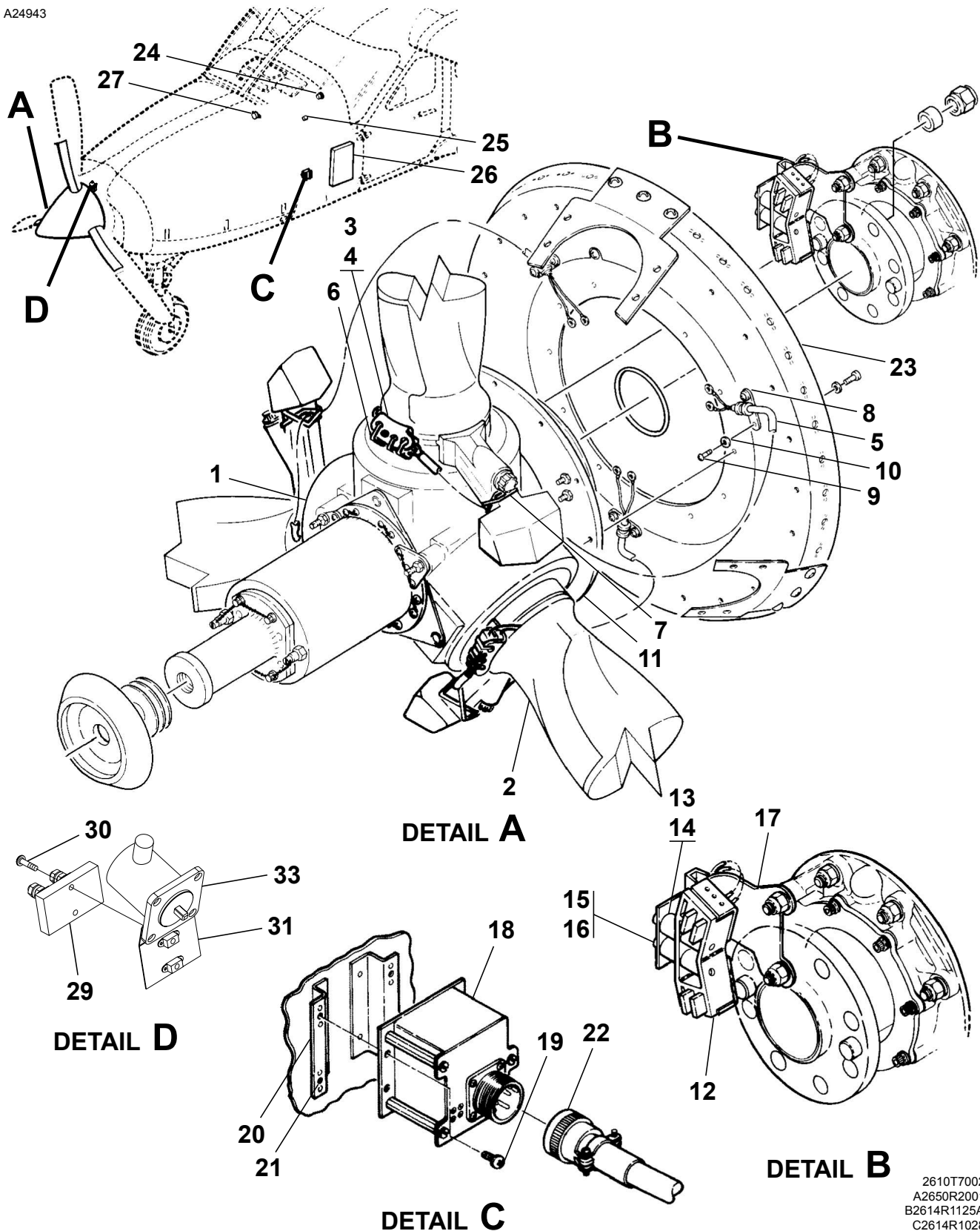
PROPELLER DEICE INSTALLATION - MCCAULEY Figure 02. (Sheet 1)
