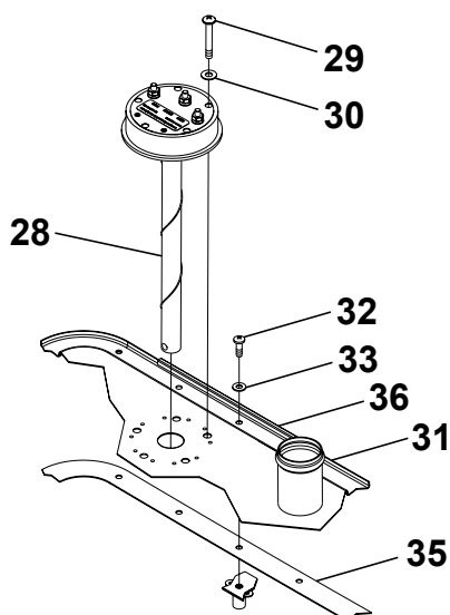
DETAIL D
