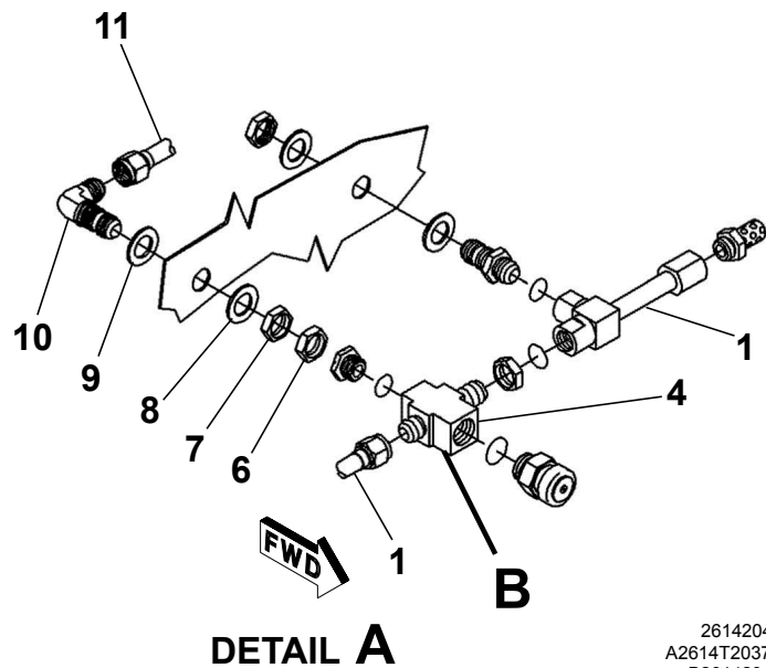
DEICE SYSTEM Figure 02. (Sheet 1)
