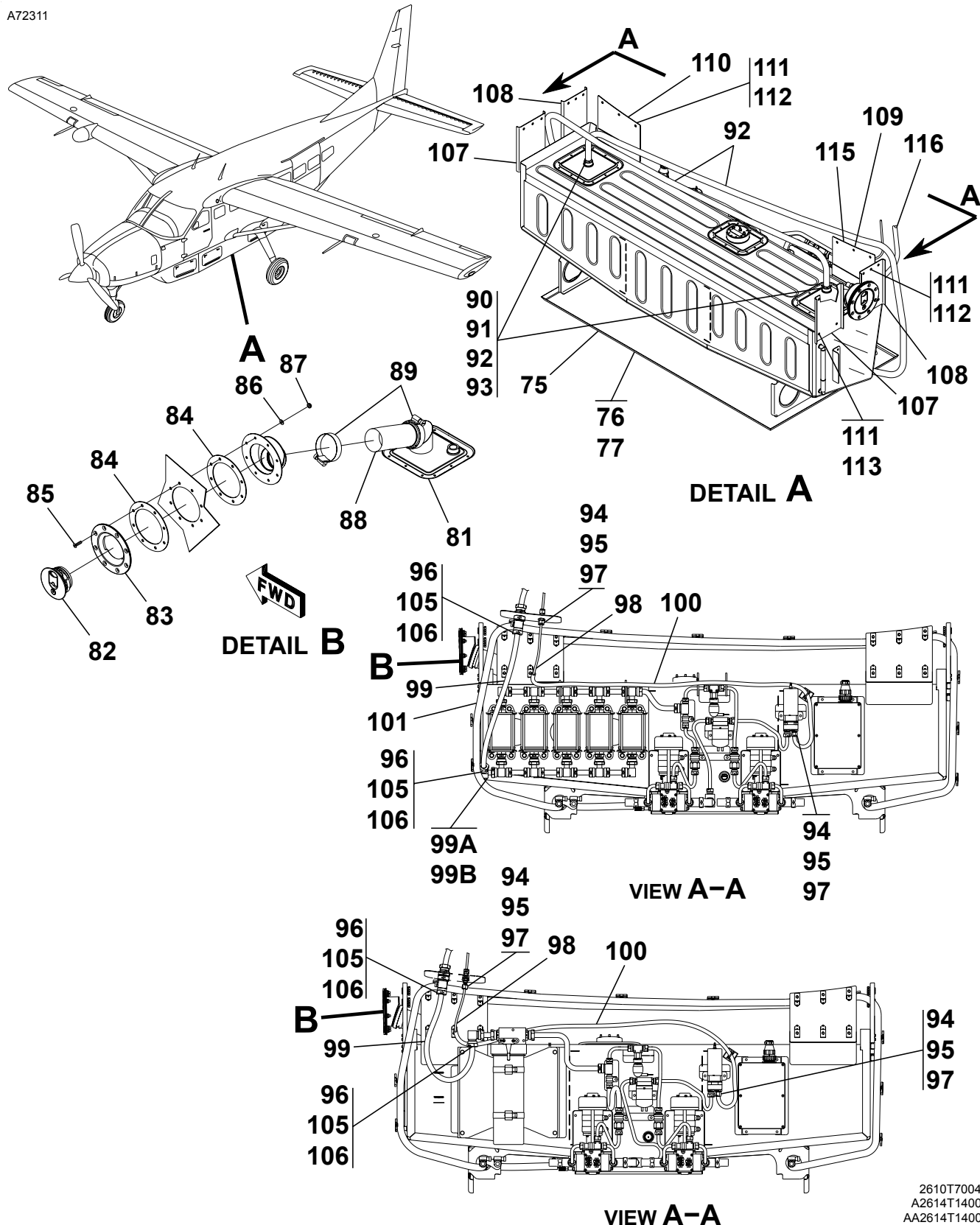
TKS FLUID TANK & EQUIPMENT PACK INSTALLATION Figure 08. (Sheet 2)
