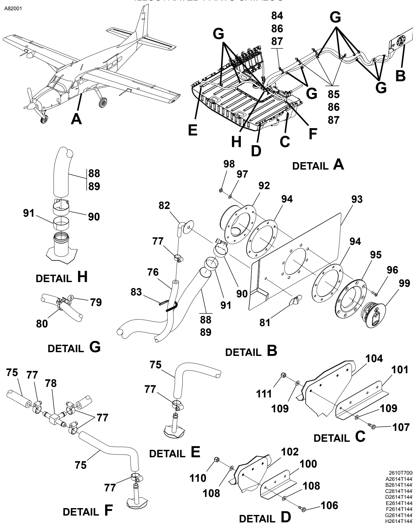
TKS LOW PROFILE TANK INSTALLATION - 208B Figure 07. (Sheet 2)
