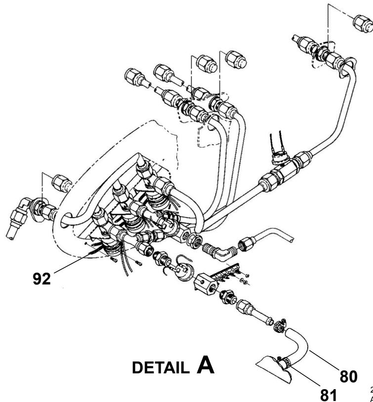
DEICE COMPONENTS - WING Figure 01. (Sheet 2)
