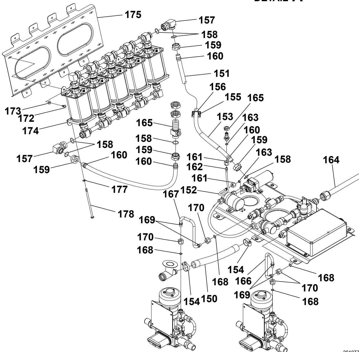
DETAIL B
