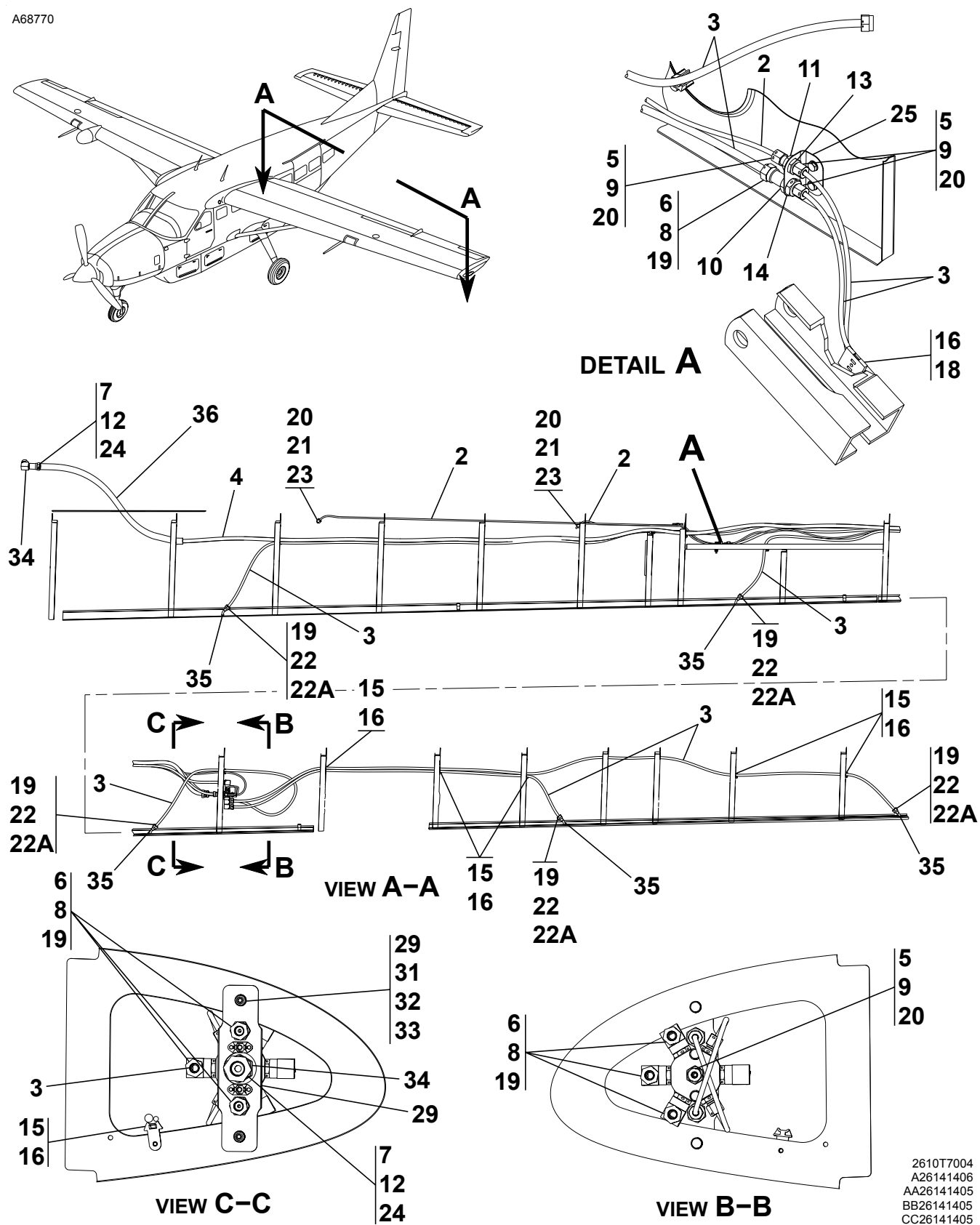
TKS TUBE ROUTING - WINGS Figure 03. (Sheet 1)
