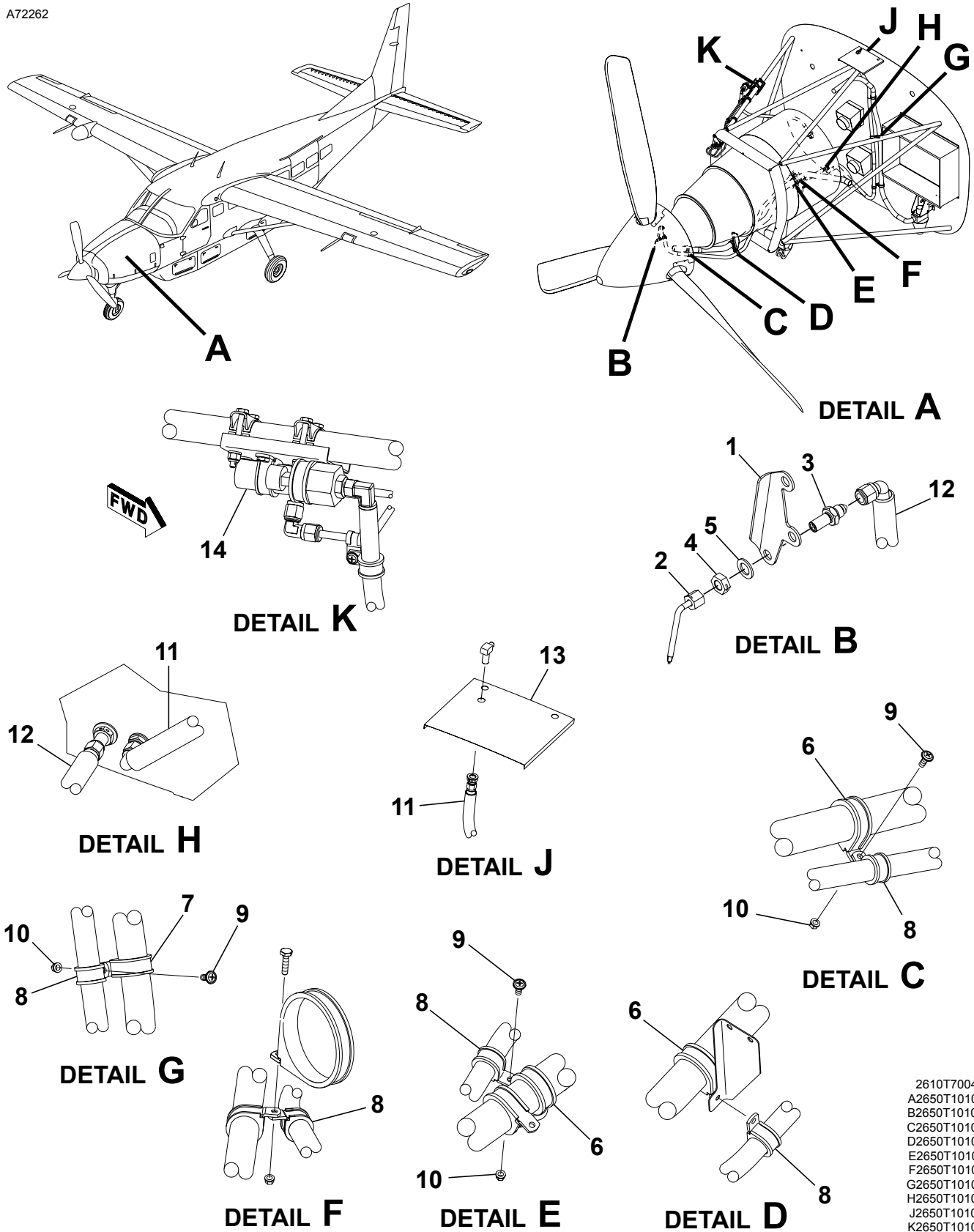
TKS FIREWALL FORWARD INSTALLATION Figure 05. (Sheet 1)
