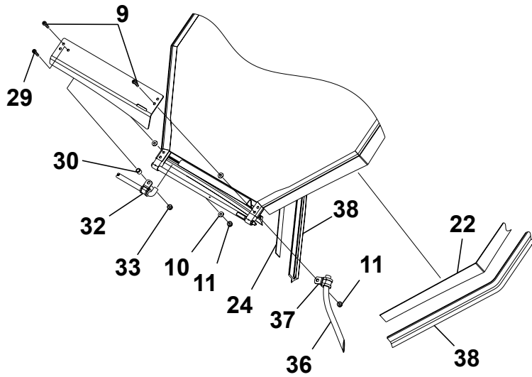
DETAIL E
