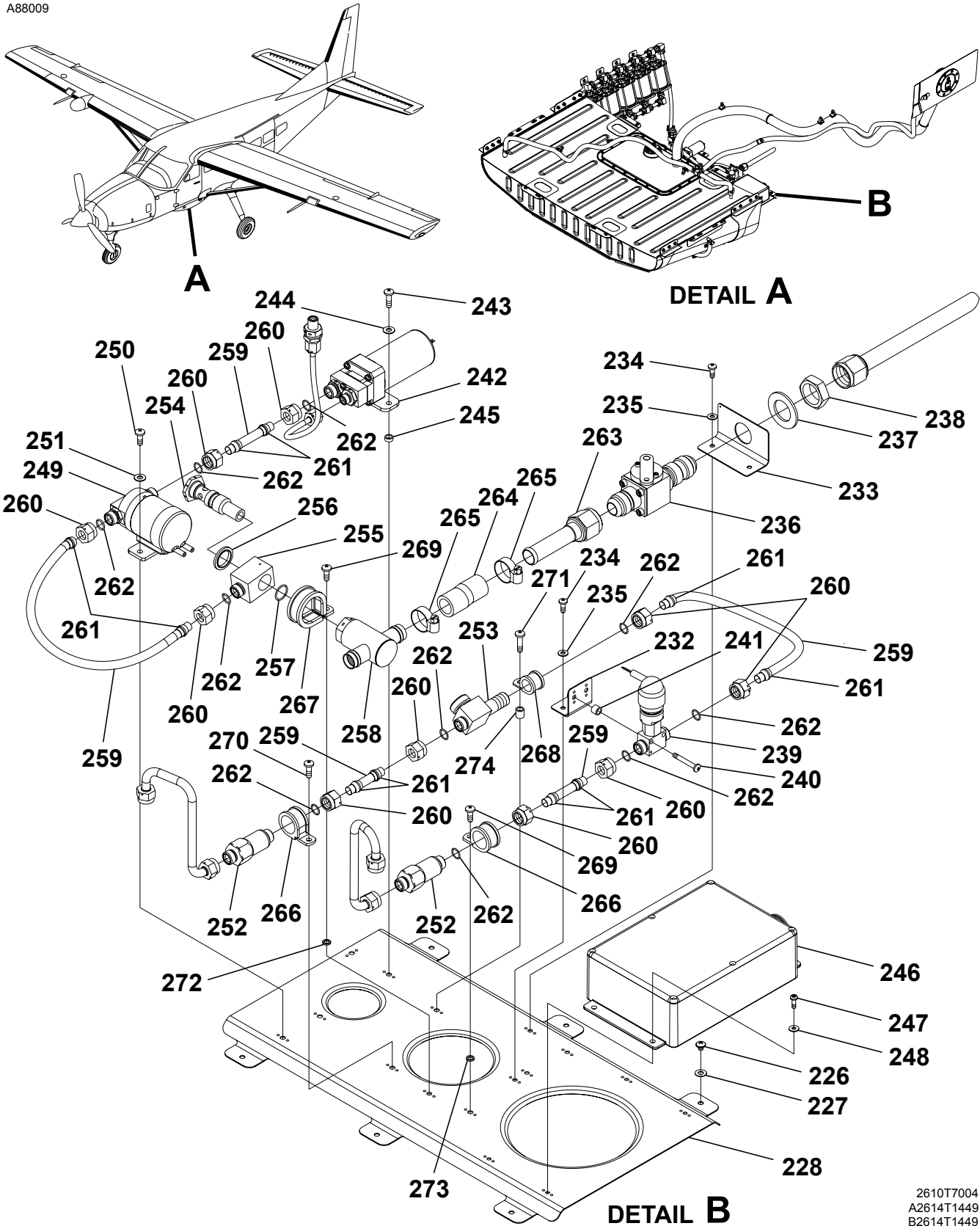
TKS LOW PROFILE TANK INSTALLATION - 208 Figure 06. (Sheet 4)
