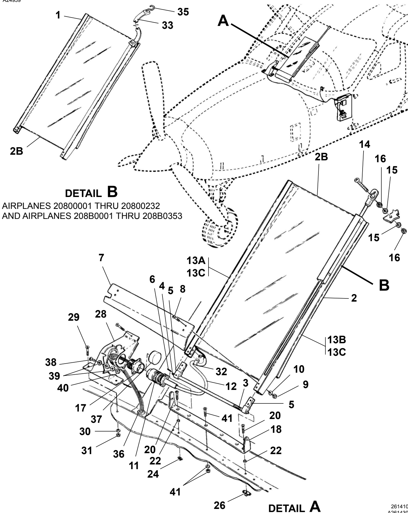
WINDSHIELD ANTI-ICE INSTALLATION Figure 01. (Sheet 1)
