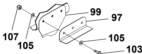
DETAIL D
