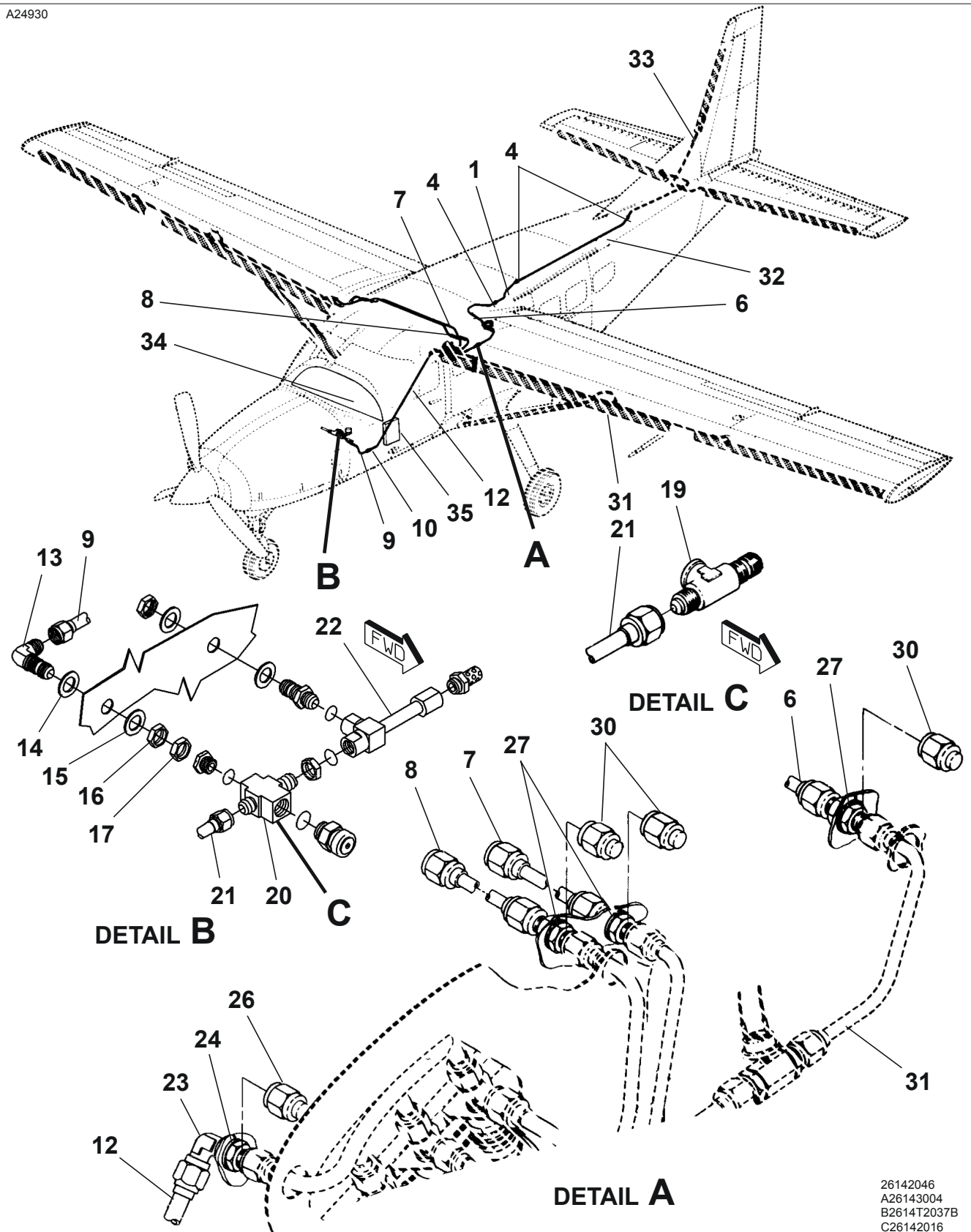
DEICE SYSTEM Figure 01. (Sheet 1)
