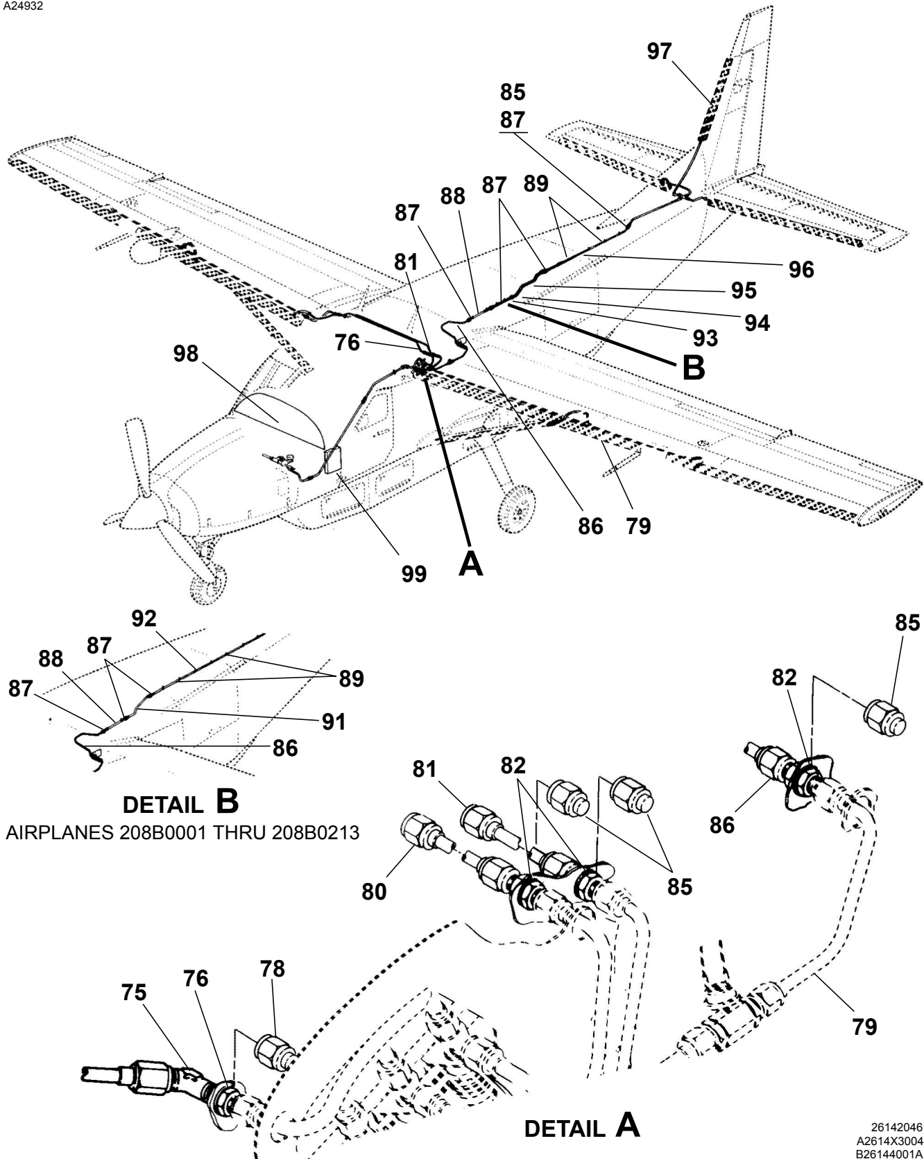
DEICE SYSTEM Figure 02. (Sheet 2)
